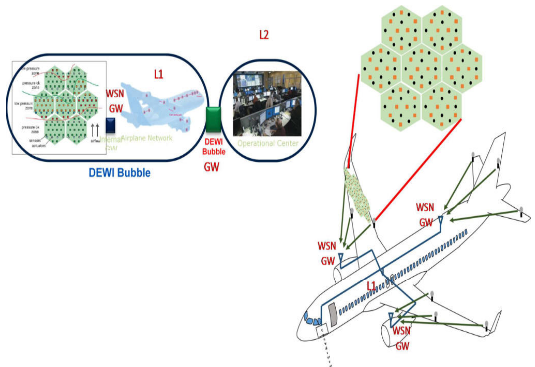
Figure 18. Mapping UC2.5 to the layered model of the DEWI HLA.
