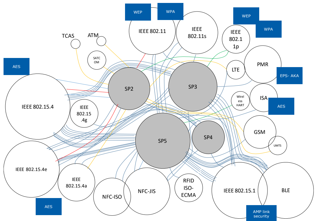
Figure 4. Wireless standards used in DEWI with some security features. SP2-Aeronautics, SP3 Automotive, SP4 Railway, SP5 Building.
