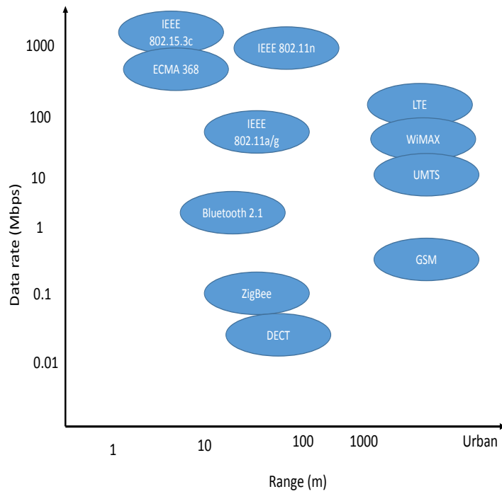
Figure 3. Data rate vs. range comparison for different wireless commercial standards L0 HLA.
