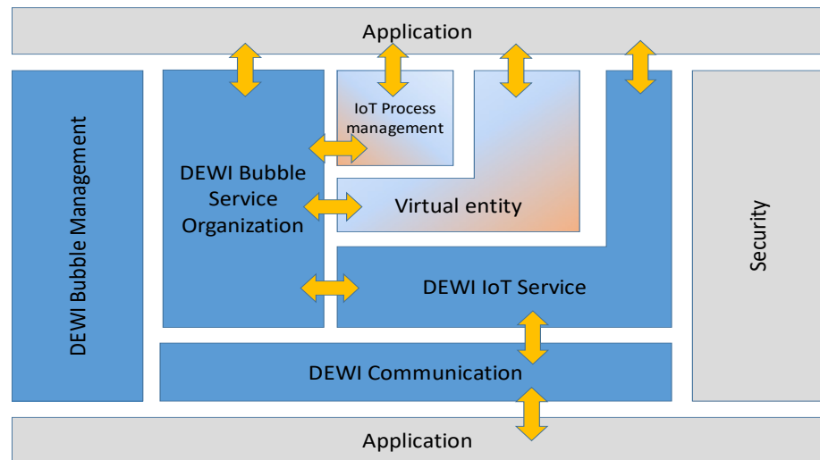
Figure 21. Mapping DEWI HLA to the IoT ARM.
