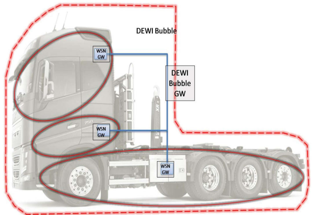
Figure 19. Mapping UC3.8 to the layered model of the DEWI HLA.
