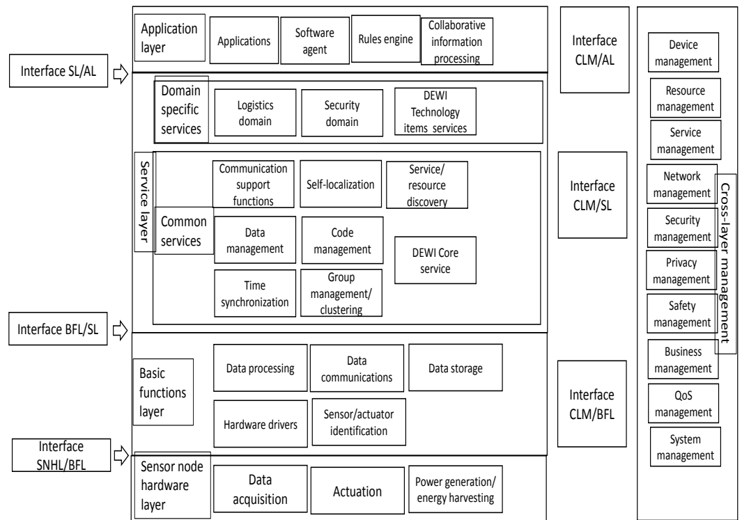
Figure 16. Protocol stack view of functional model of the DEWI/ISO HLA.
