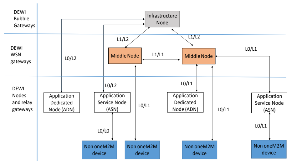
Figure 22. Mapping DEWI HLA to the oneM2M architecture.
