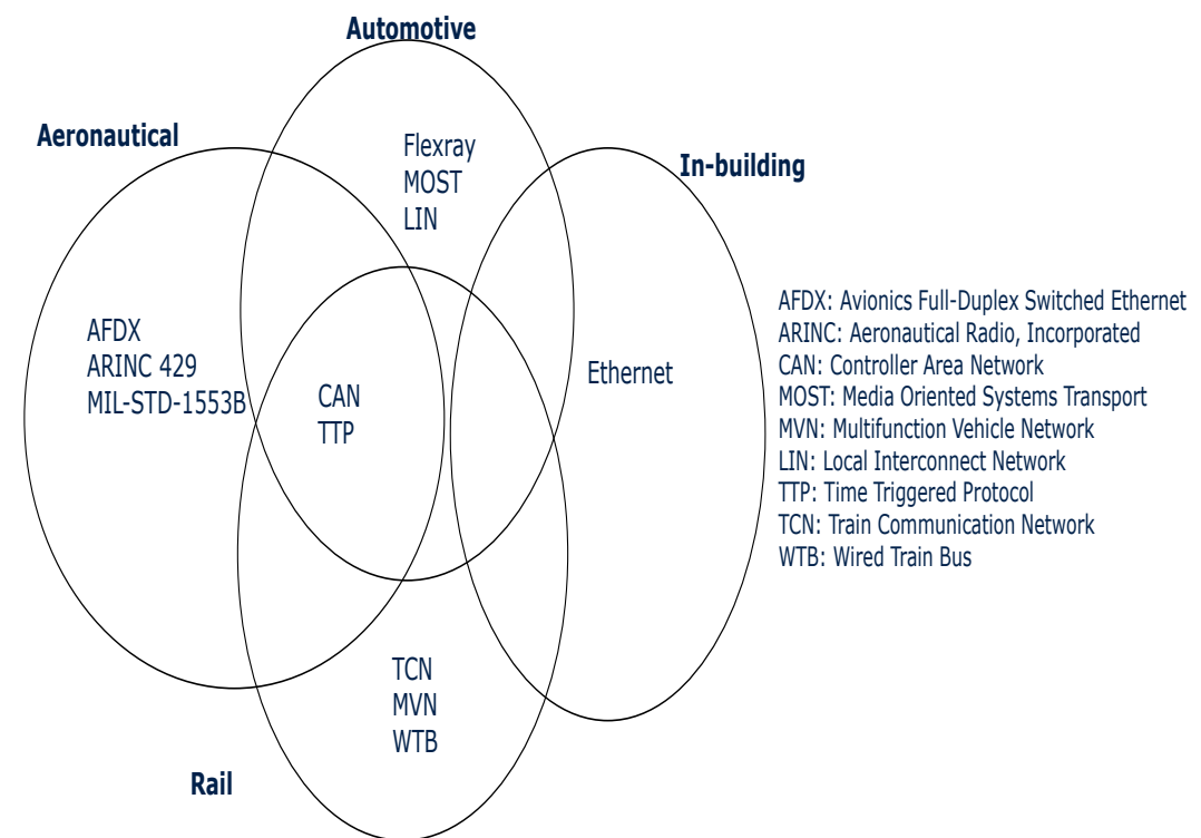
Figure 9. L1 industrial wireline technologies. SP2-Aeronautics, SP3 Automotive, SP4 Railway, SP5 Building.
