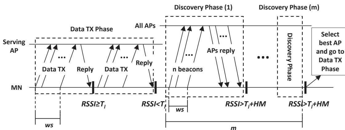
Figure 3.1: Timing diagram of the smart-HOP mechanism, illustrating the two phases and the messages exchanged.
