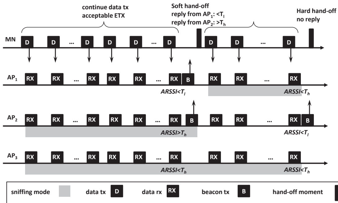
Figure 7.2: An example of mRPL+ with three APs and a MN. The x-axis illustrates the order of the processes in mRPL+, considering data/control message exchanges and hand-off mechanism.
