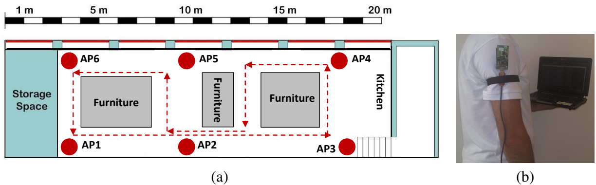
Figure 4.7: (a) The APs' deployment in a large room, and (b) the MN attached to a person's arm and the logging PC [FAZK14].
