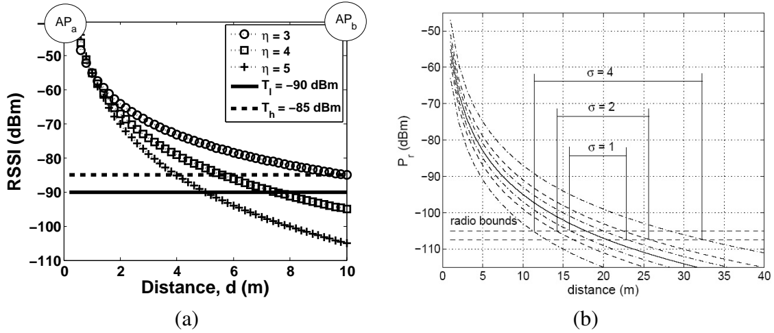
Figure 4.3: Impact of channel parameters on the RSSI with T_\ell = -90 dBm and HM=5 dBm, (a) impact of path-loss exponent on RSSI [FAZK14], and (b) impact of shadow fading on the RSSI ( P_r indicates the received signal strength) [ZK04].
