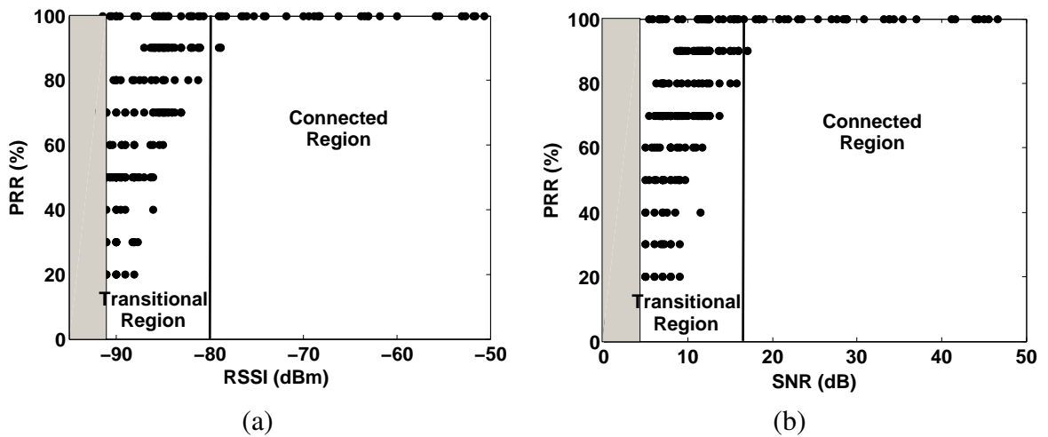
Figure 1.3: Low-power link model (a) RSSI vs. PRR. For RSSI greater than -80 dBm, the PRR is greater than 90%, and for RSSI less than -92 dBm, the PRR is less than 10%. In between, a small variation in the RSSI can cause a big difference in the PRR, which is identified as transitional region. (b) SNR vs. PRR. The borders for SNR are 4 dB and 16 dB, which are obtained by subtracting the noise floor from the RSSI readings [FZA + 12].
