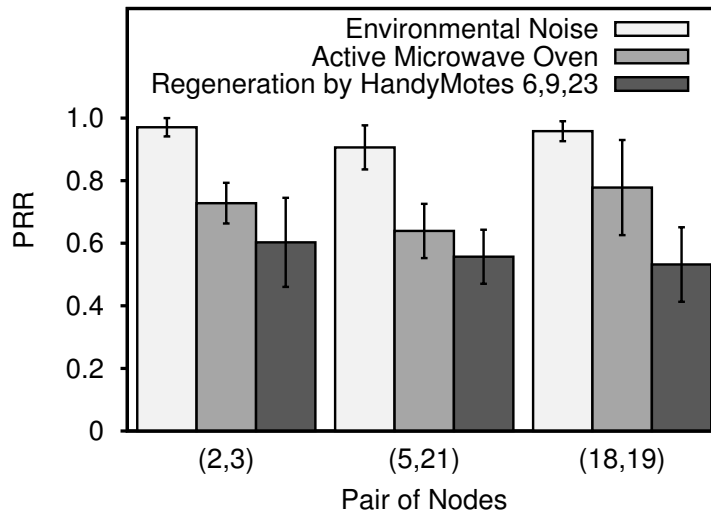
FIGURE 2.12: Comparison of the PRR obtained generating interference using a microwave oven and using JamLab.
