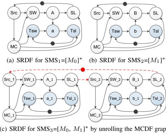
Fig. 4. The equivalent SRDF of recurring SMS for the MCDF in Fig. 3.
