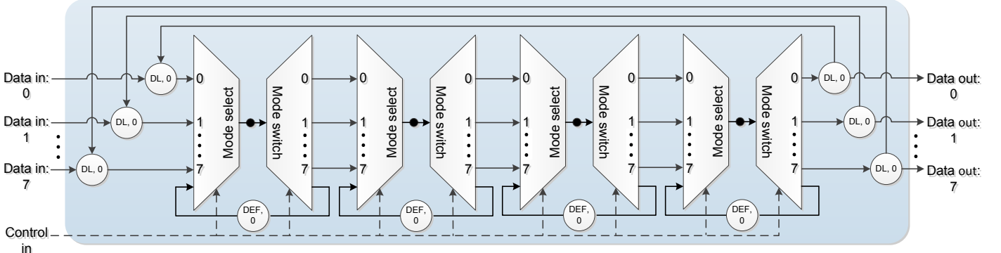
Fig. 11. A cascade tunnel structure to support multiple initial tokens for a specific set of modes.
