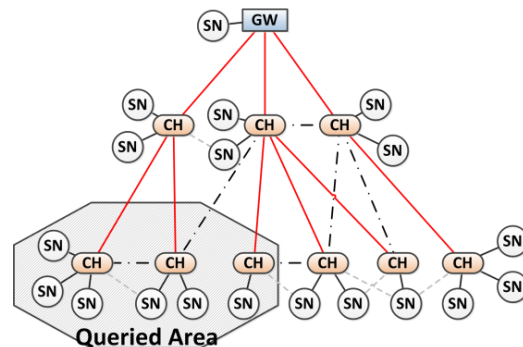
Figure 3 – Cluster Tree of a WSN Patch. Continuous line indicates Parent-Child relations; dashed line stresses that deployment planning should allow for a child to have alternative parents.
