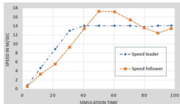
Fig. 4: Leader and the follower vehicle moving without any braking. The leader with a Target speed of 50km/h (13.8m/s) and the Follower oscillating to keep up with the target speed while maintaining the inter-vehicle distance.
