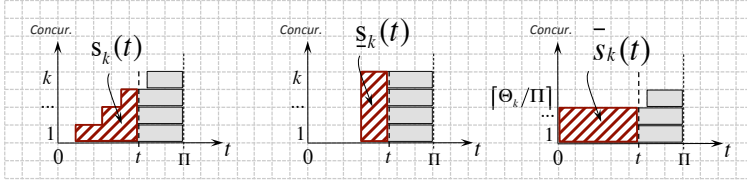
Fig. 14 The lower and upper bounds \underline{s}_k(t) , \bar{s}_k(t) for the supply function s_k(t) . The overall supply allocated over [0; II] is \Theta_k .
