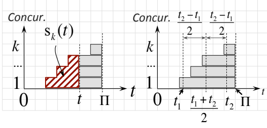
Fig. 7 Properties of the s_k(t) function.
