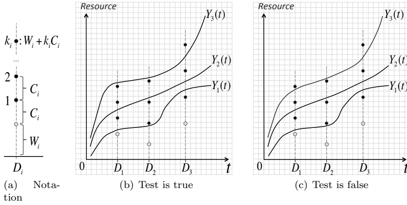
Fig. 16 Graphical interpretation of the PSF-based schedulability test
