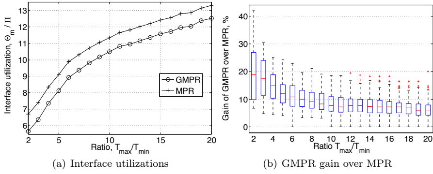
Fig. 19 Case: U_{\mathcal{T}} = 2.5 , U_{\max} = 0.3 , \Delta m = 3 , \Pi = 20 .
