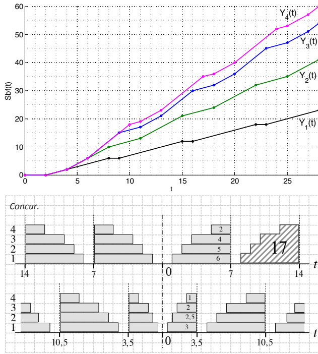
Fig. 13 The PSF (top) and the worst-case supply patterns (bottom) of the GMPR interface \langle 7, \{6, 11, 15, 17\} \rangle . The bold points indicate the slope change of the PSF functions.
