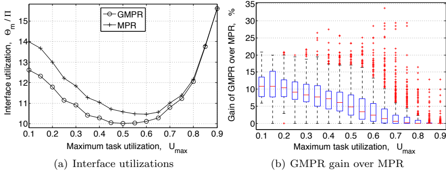
Fig. 18 Case: U_{\mathcal{T}} = 2.5 , \frac{T_{\max}}{T_{\min}} = 10 , \Delta m = 3 , \Pi = 20 .
