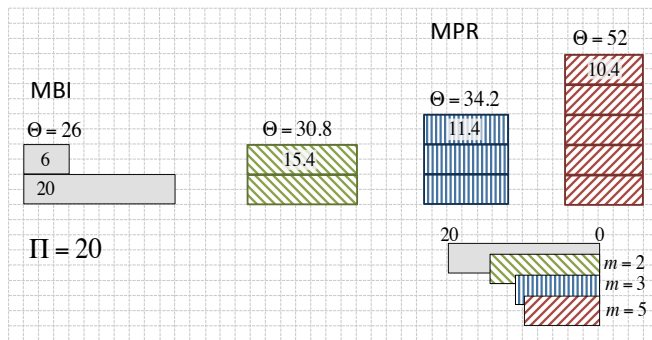
Fig. 3 Comparison of MBI and MPR
