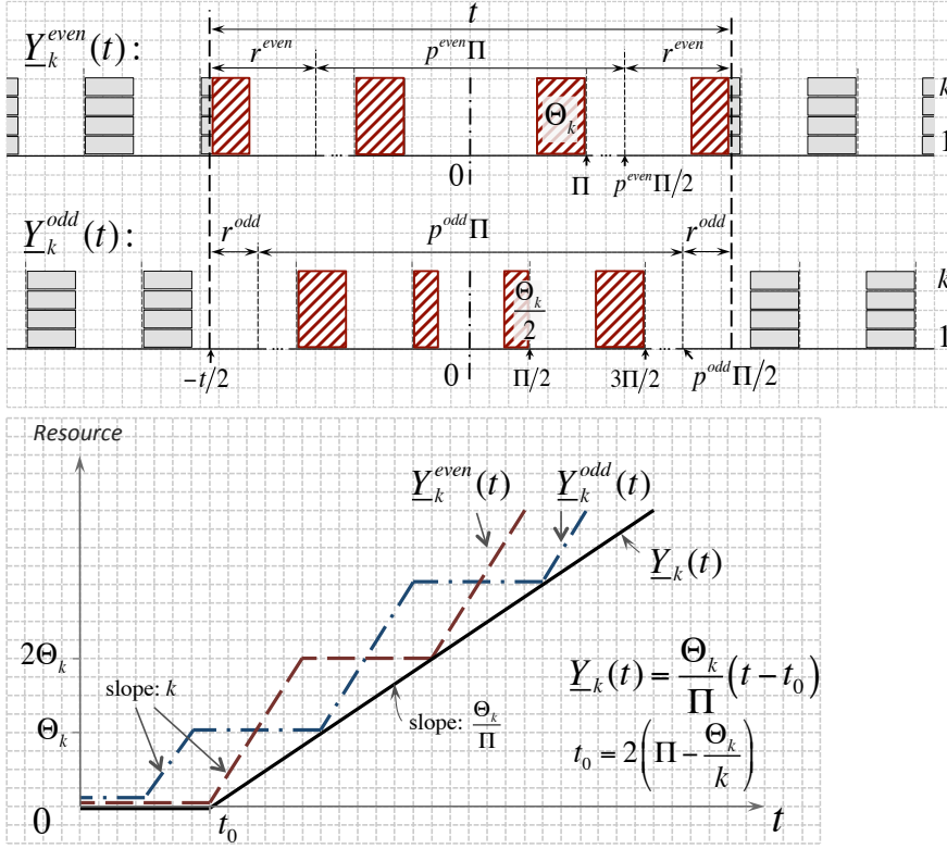
Fig. 15 The lower bound for Y_k(t) .
