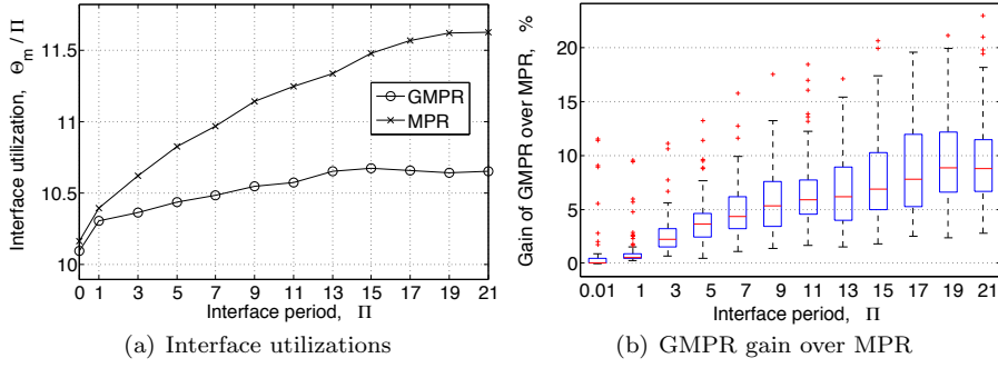
Fig. 17 Case: U_{\mathcal{T}} = 2.5 , U_{\max} = 0.3 , \frac{T_{\max}}{T_{\min}} = 10 , \Delta m = 3 .
