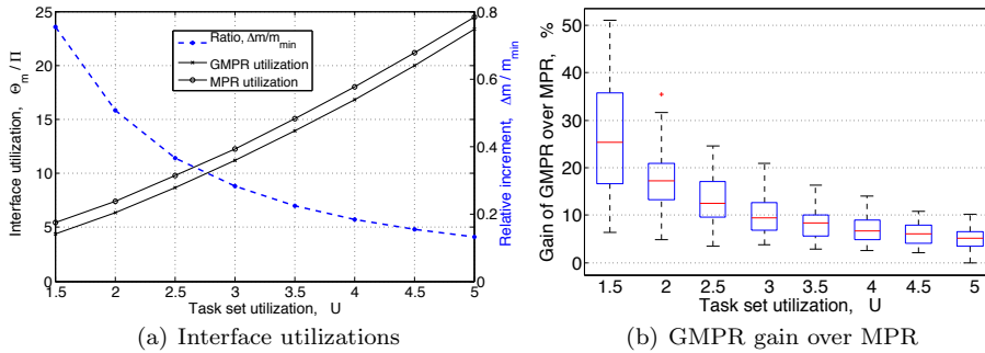
Fig. 20 Case: U_{\max} = 0.3 , \frac{T_{\max}}{T_{\min}} = 10 , \Delta m = 3 , \Pi = 20
