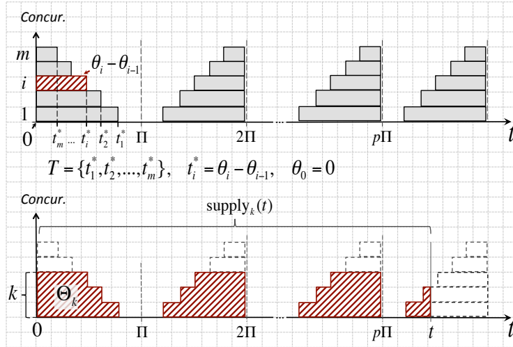
Fig. 6 The worst-case resource allocation over GMPR \langle \Pi, \{\Theta_1, \dots, \Theta_m\} \rangle (top) and the definition of the \text{supply}_k(t) function (bottom) proposed by Burmyakov et al (2012).
