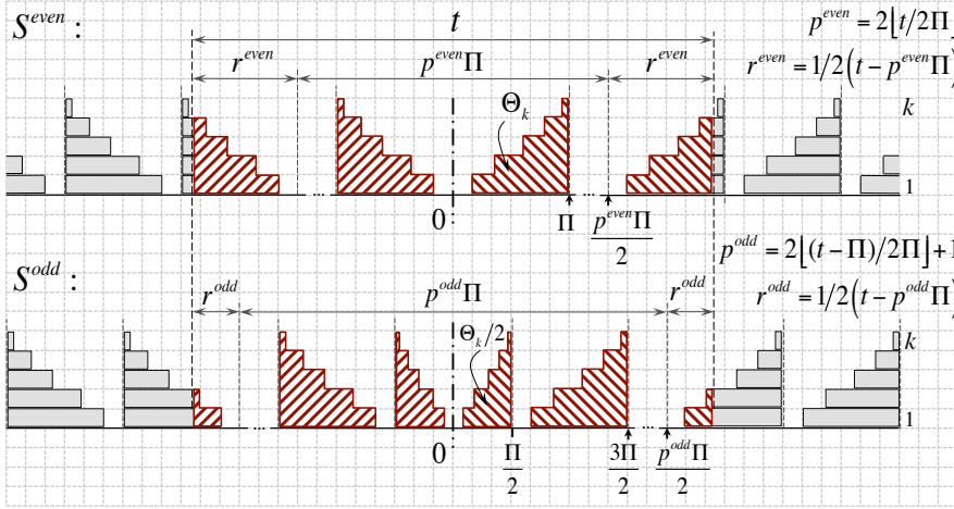
Fig. 8 The worst-case resource allocation patterns S^{\text{even}} and S^{\text{odd}} over GMPR \langle \Pi, \{\Theta_1, \dots, \Theta_m\} \rangle .
