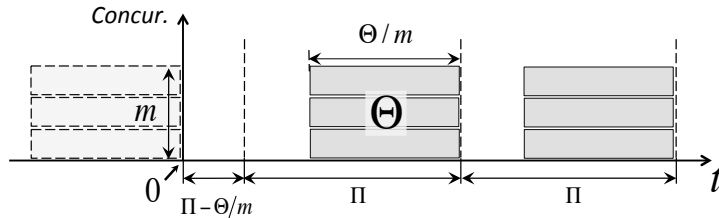
Fig. 2 The worst-case resource allocation over the MPR \langle \Pi, \Theta, m \rangle . Instant 0 denotes the beginning of the worst-case interval.
