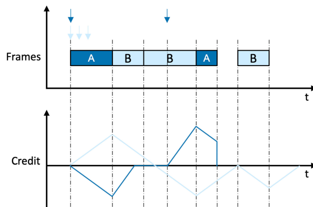
FIGURE 1. Example of the operation of the Credit Based Shaper, reproduced as in [27].
